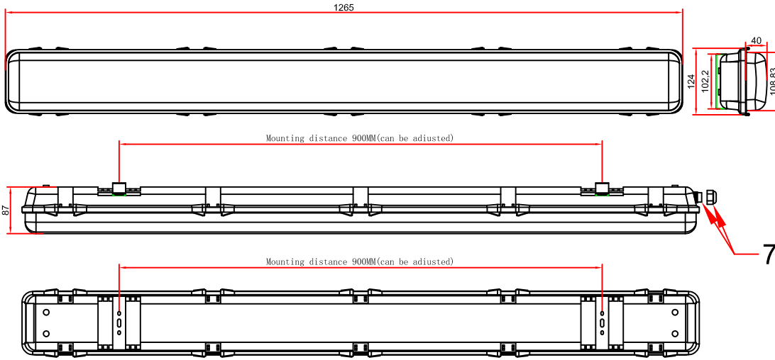
Details Drawing
